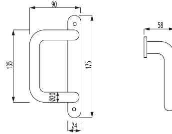
02 - 146 Rozetli Sosis Kol Cylindrical Door Handle & Carpet
