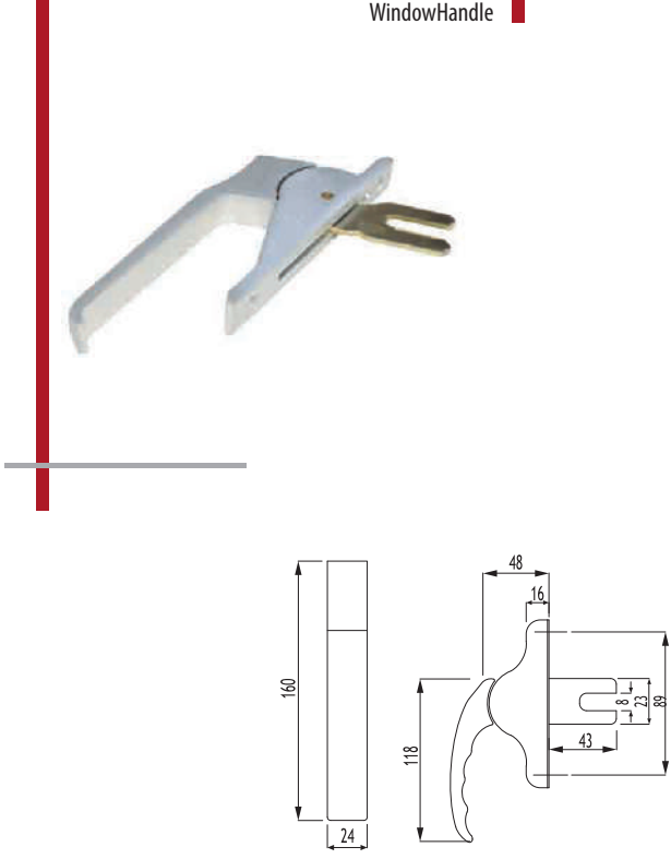
02 - 153 Kıvrık Cephe Kolu Tek Dilli Facede Window Handle
